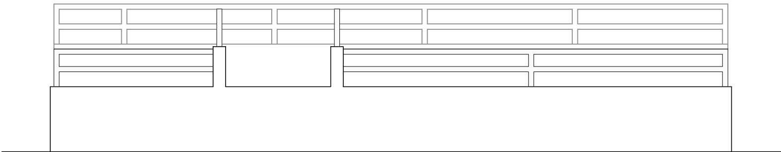
Fachada Frontal – Curral Bovino escala + 1/75
